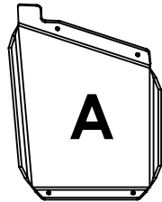
42054 (A) Left End Skid Shoe 11" X 15" (4) 5/16-18 x 3/4 Carriage Bolt (4) 5/16-18 Flange Nut
