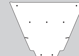
Center Skid Shoe 17 1/4" x 23" 41567 - 3/8"
