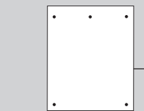
Left End Skid Shoe 3" x 8 1/2" 42056 - 3/8"
